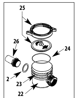
DETAIL 7
